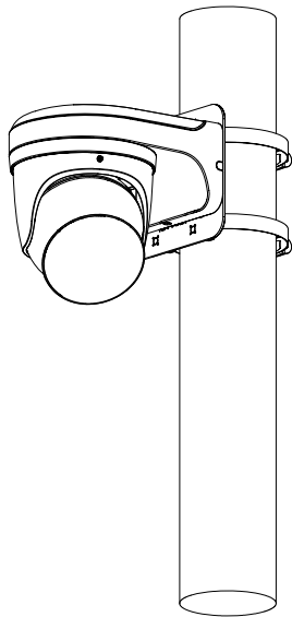
Pole Mount(Vertical)
