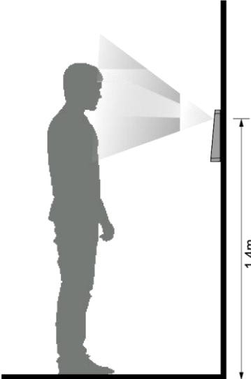
Figure 2-6 Installation diagram
