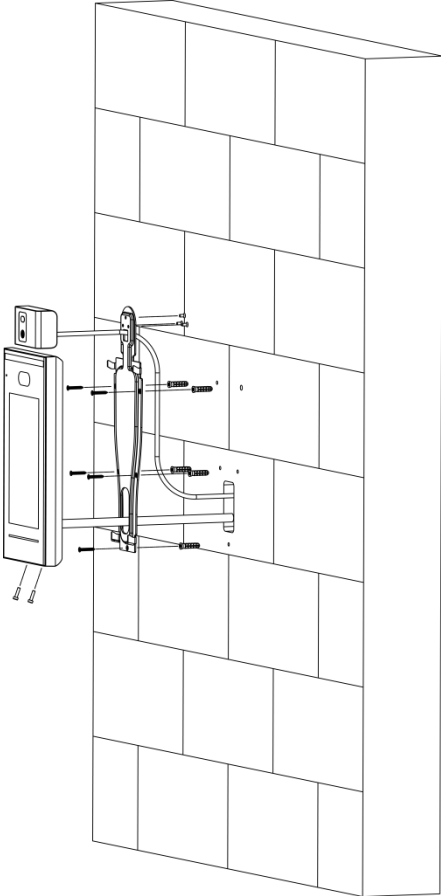
Figure 2-6 Installation diagram
