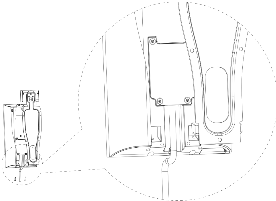
Figure 2-7 Applying silicon sealant
