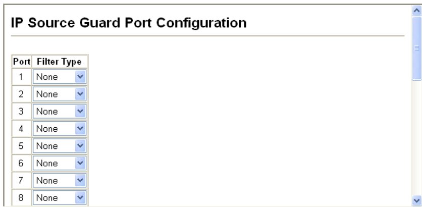
Figure 3-75 IP Source Guard Port Configuration
