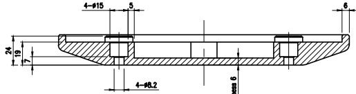
SEC BB
