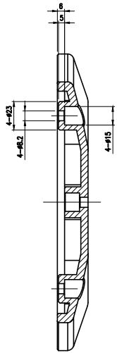
SEC AA
